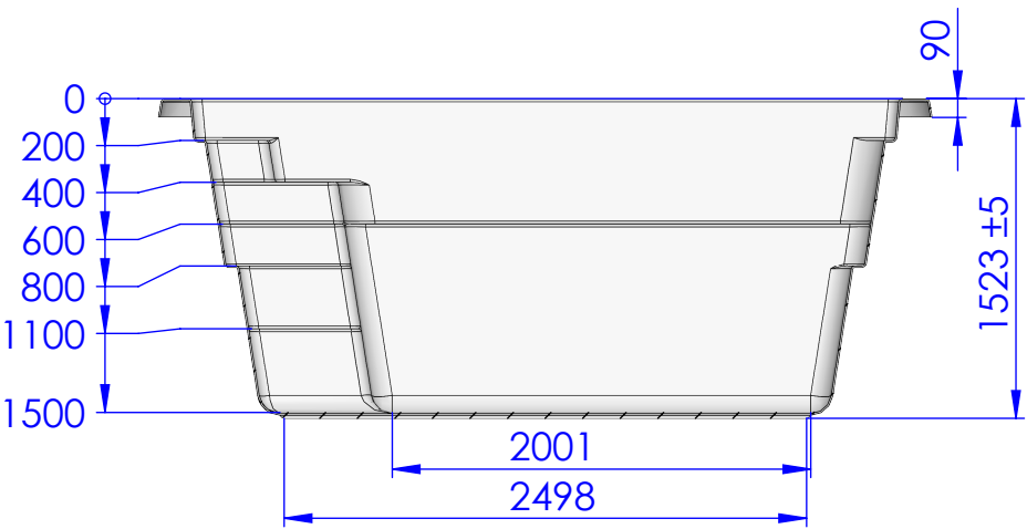
SECTION B-B SCALE 1 : 40
