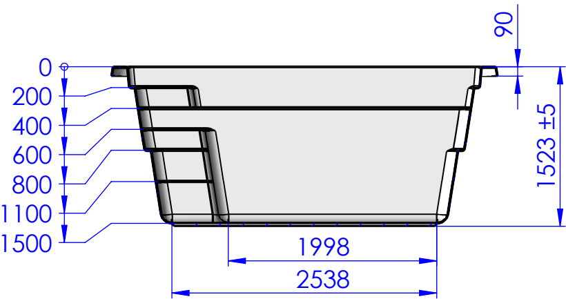
SECTION B-B SCALE 1:45
