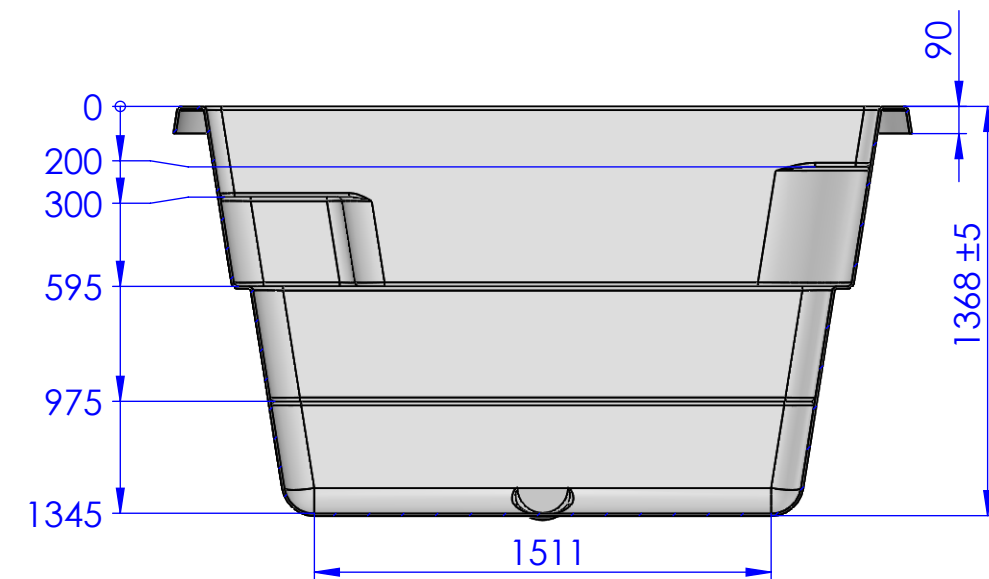
SECTION B-B SCALE 1 : 25
