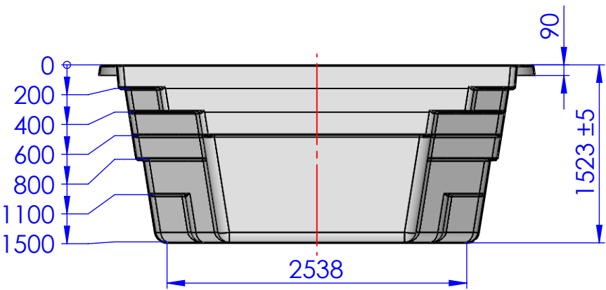
SECTION B-B SCALE 1 : 45
