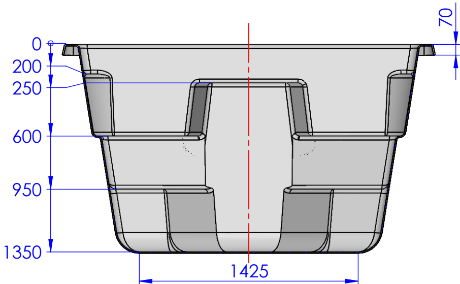
SECTION B-B SCALE 1 : 25
